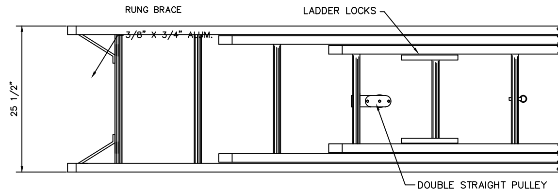
PLAN VIEW
