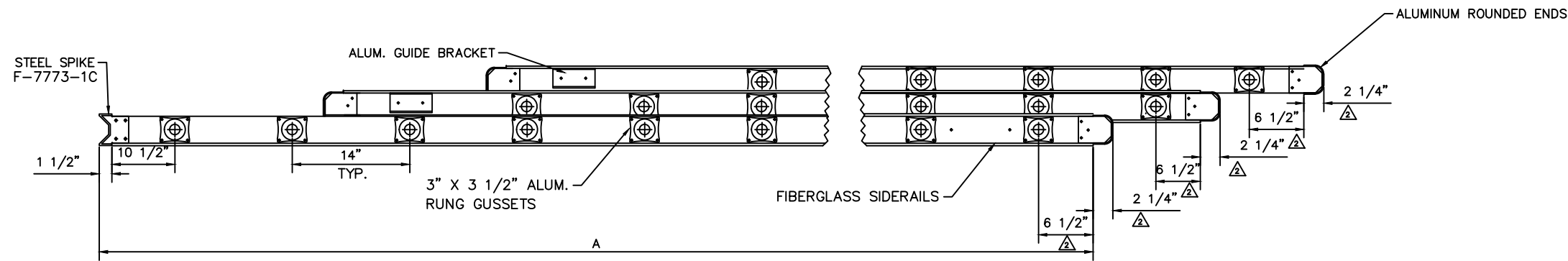
SIDE VIEW
