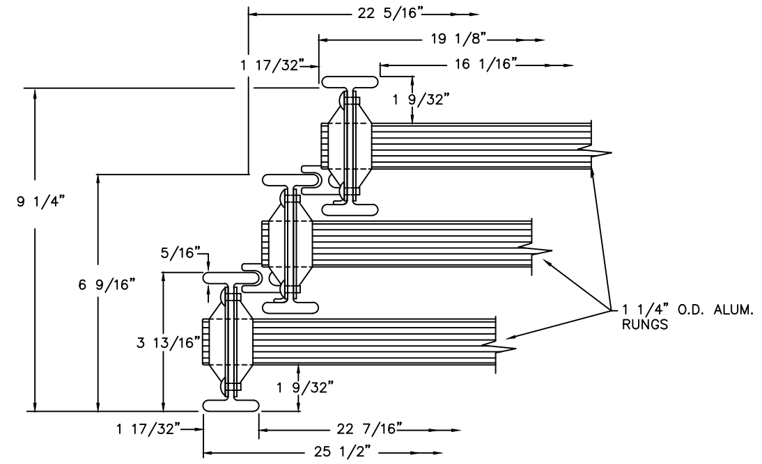
CROSS SECTION
