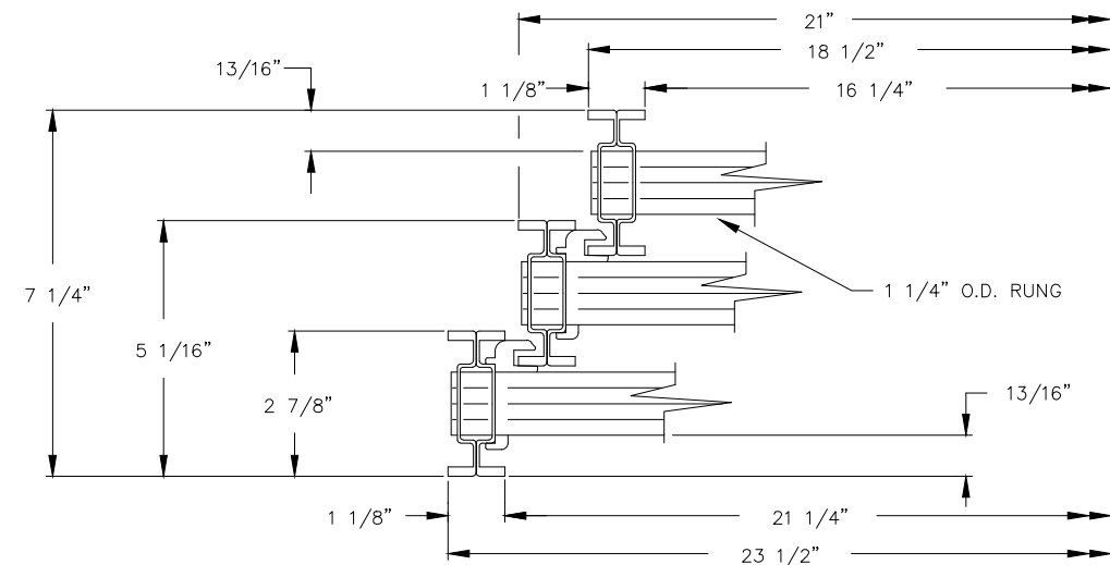
CROSS SECTION
